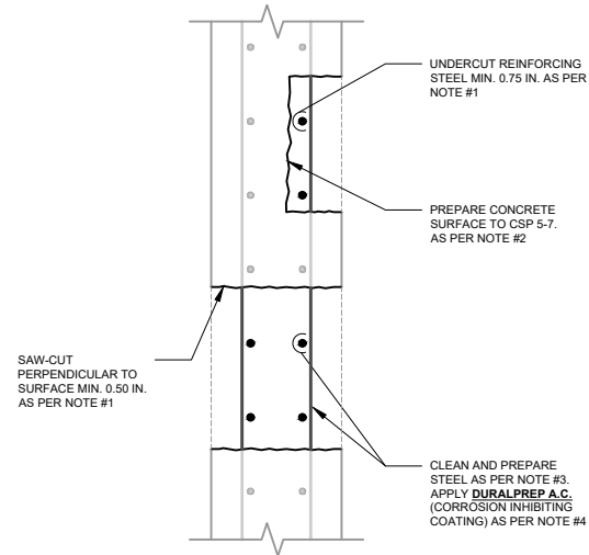
CONCRETE REMOVAL AND SURFACE PREPARATION
